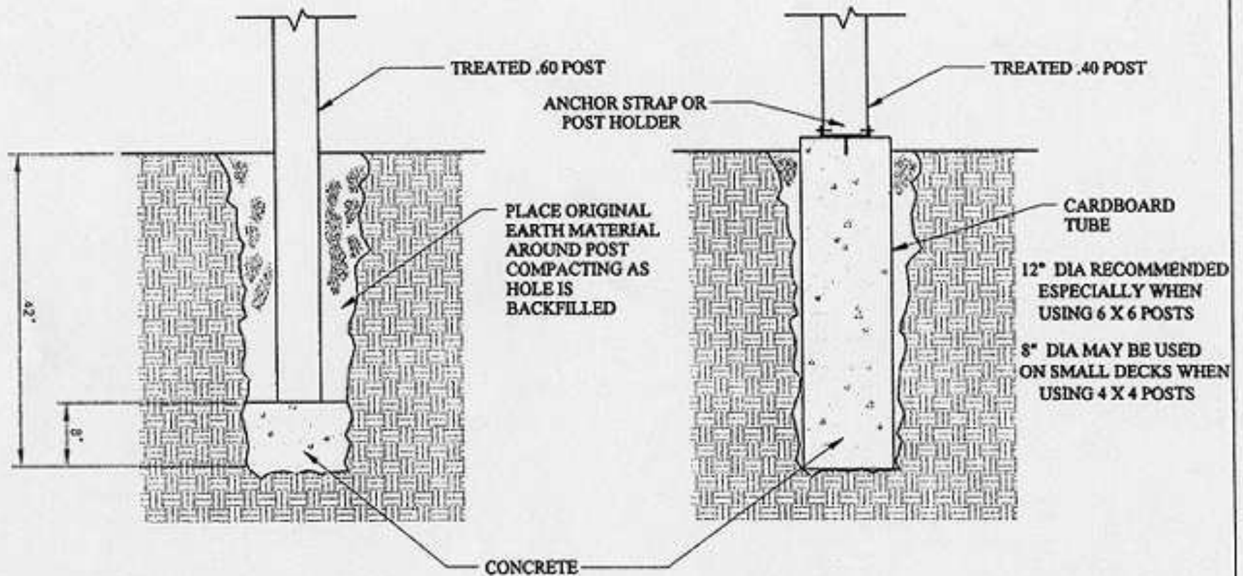
Cardboard Tube Concrete Pier Footing
